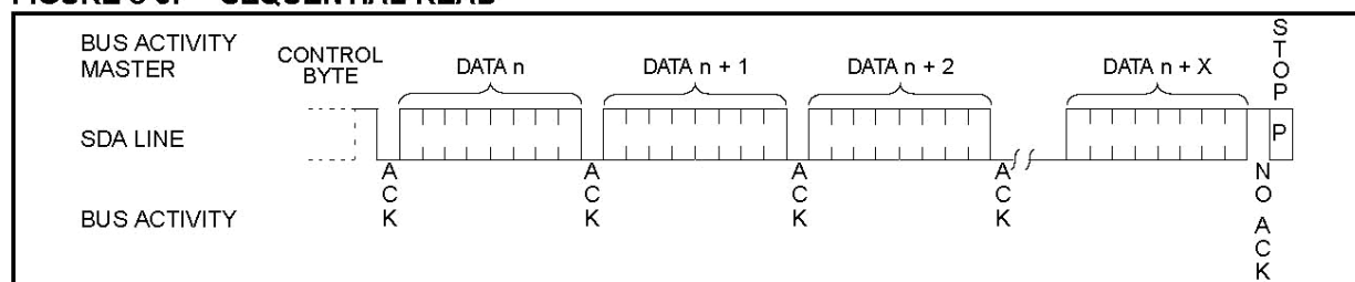
FIGURE 8-3: SEQUENTIAL READ
