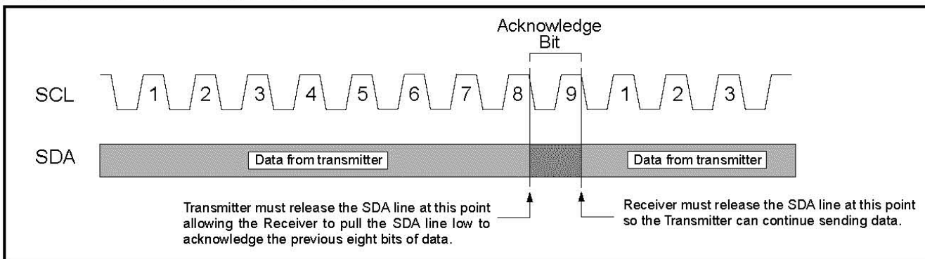
FIGURE 4-2: ACKNOWLEDGE TIMING
