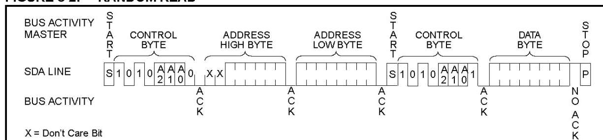
FIGURE 8-2: RANDOM READ
